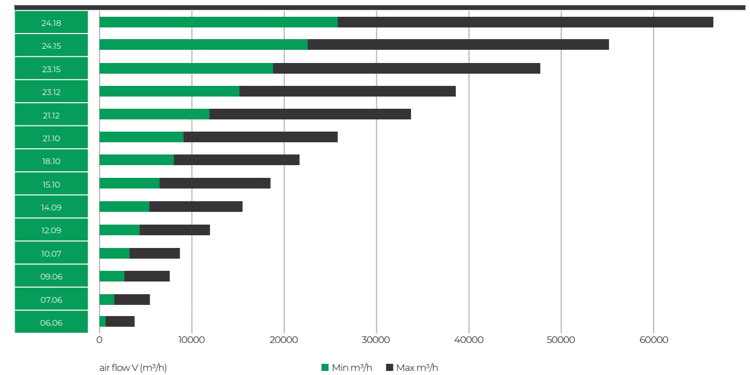
energy | pro Adiabatic Basic | AHU airflow diagram
