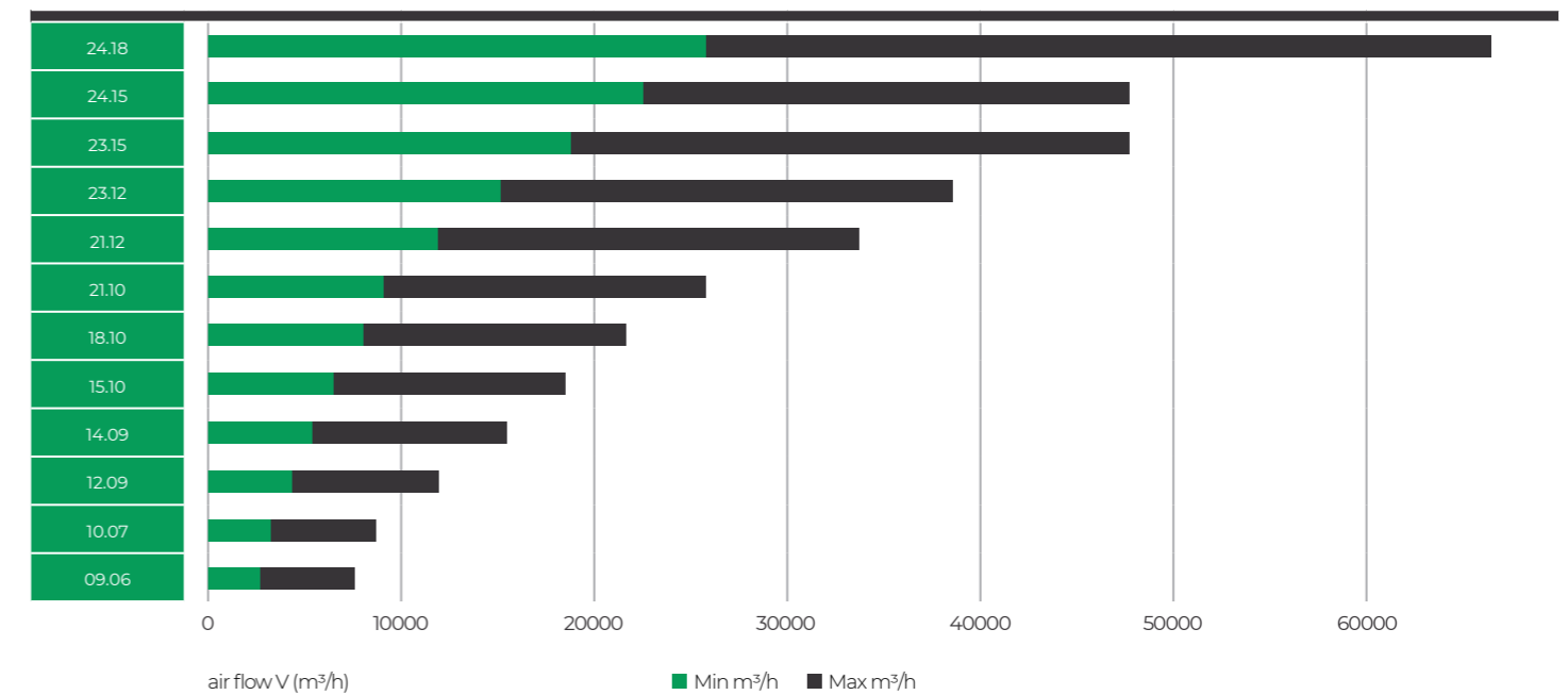
energy | pro Adiabatic Standard | AHU airflow diagram
