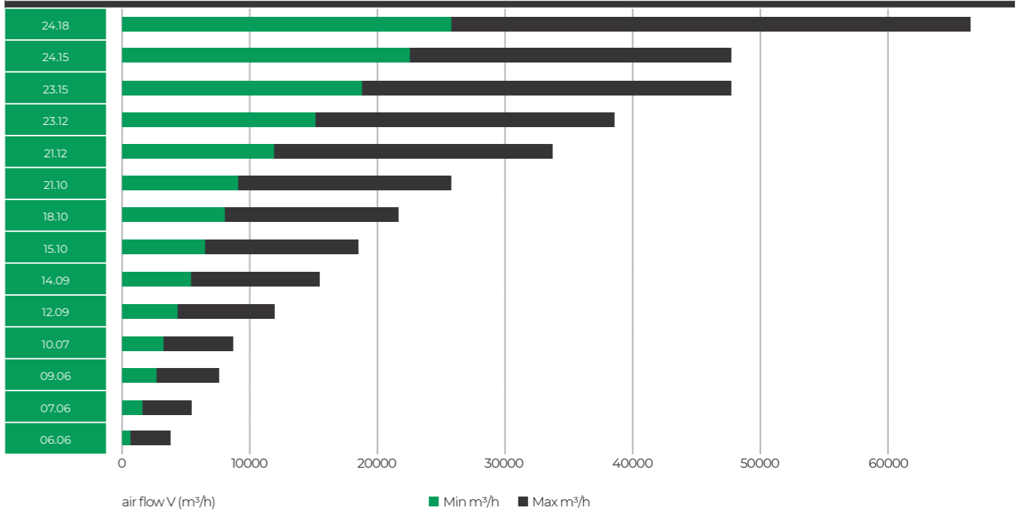
energy | pro Adiabatic Standard | AHU airflow diagram
